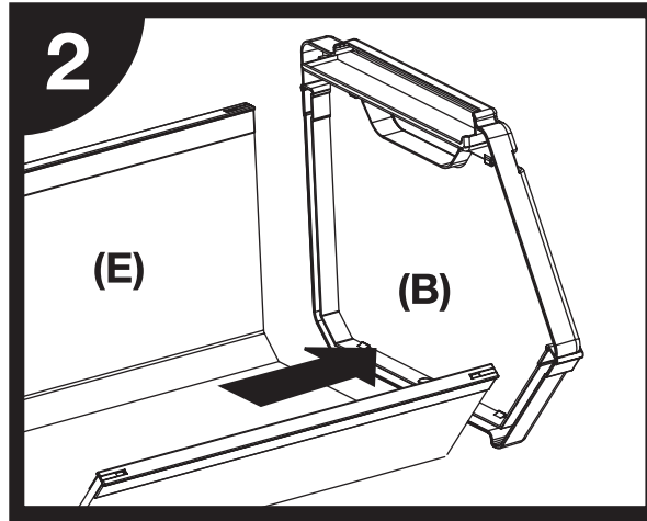
Insert body (E) into right end cap (B)
