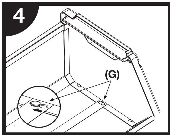
Slide keyholes on end of plastic band (G), over lugs, and lock
